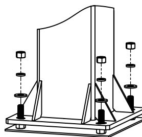
INSTALLATION VIEW MAIN POST ON J-BOLTS
