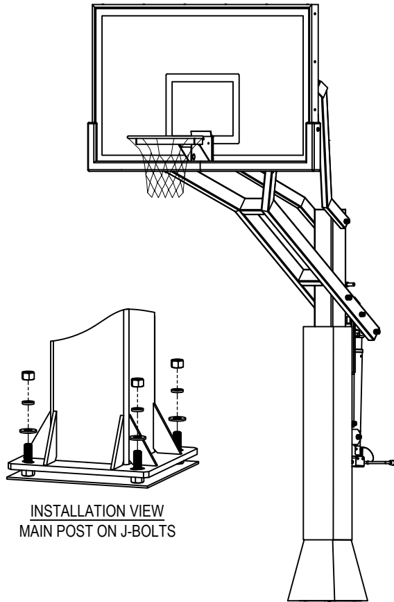
PERSPECTIVE FRONT VIEW
