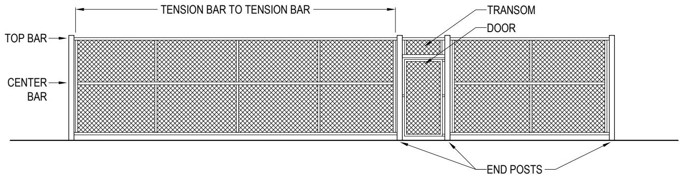
FRONT VIEW
