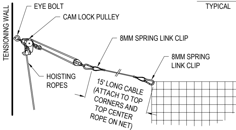
DETAIL TUNNEL TENSION KIT FROM TENSIONING WALL
