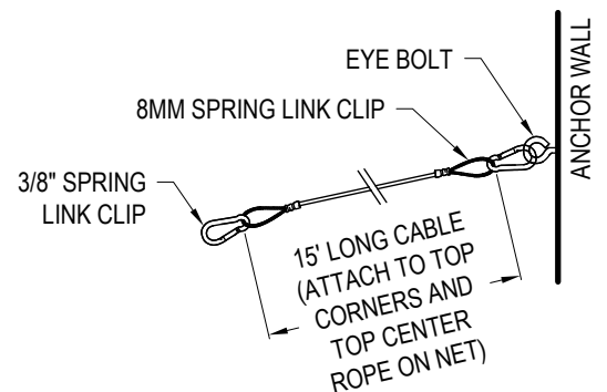
DETAIL TUNNEL TENSION KIT FROM ANCHOR WALL
