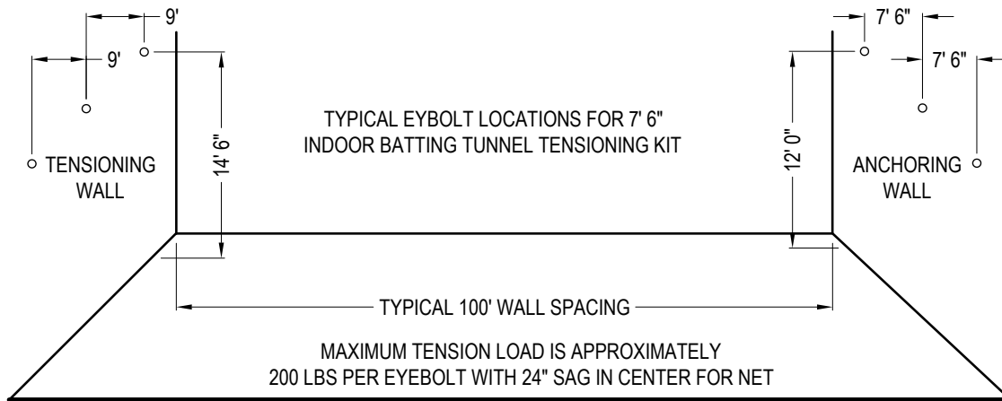
PERSPECTIVE TYPICAL
