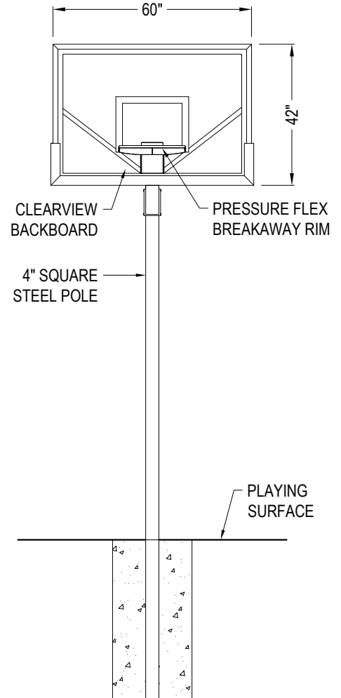
FRONT ELEVATION
