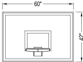
STEEL BACKBOARD FRONT ELEVATION
